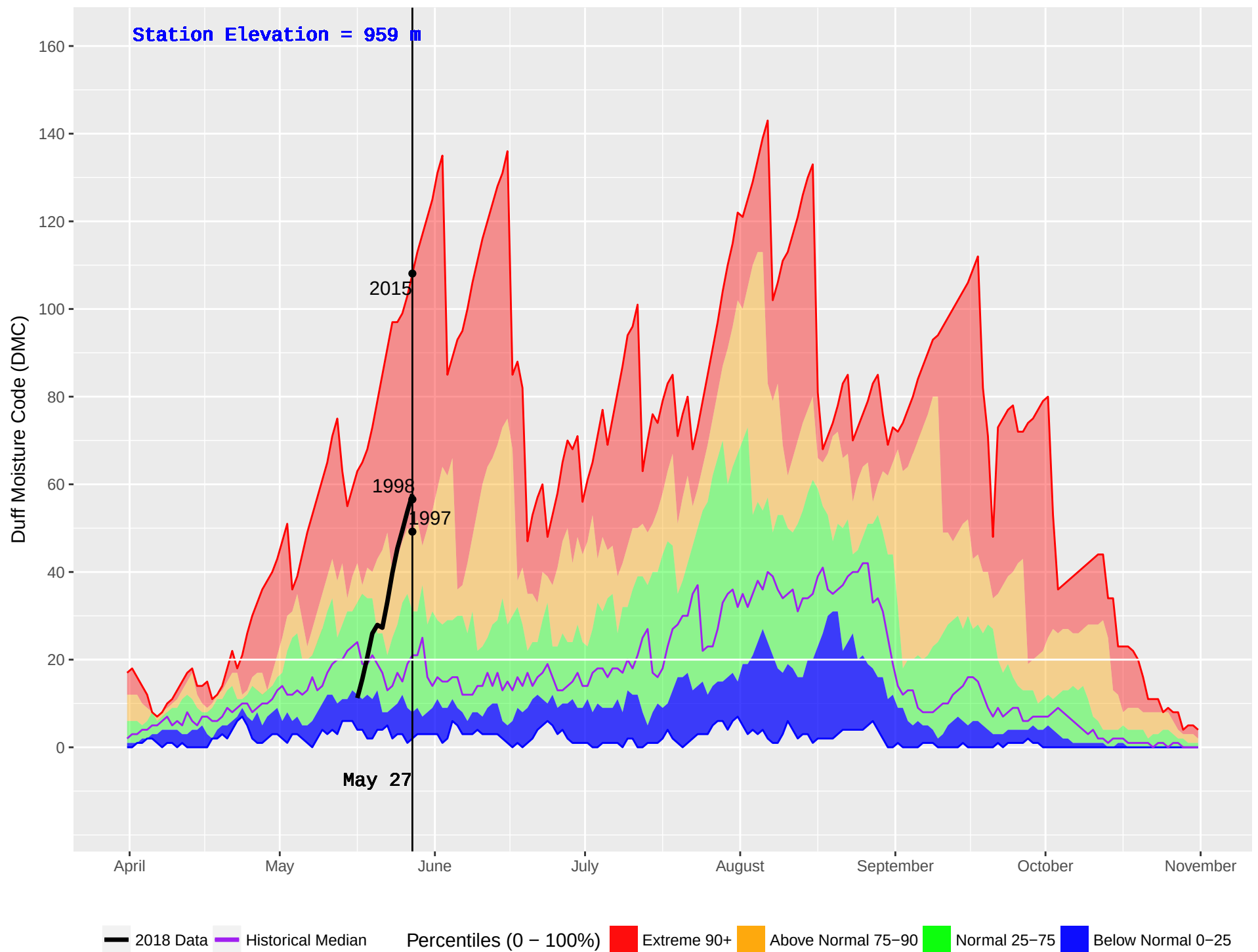
WELLS GRAY (266) : Historical (1994–2016) and Current (2018) Noon Duff Moisture Code (DMC)
