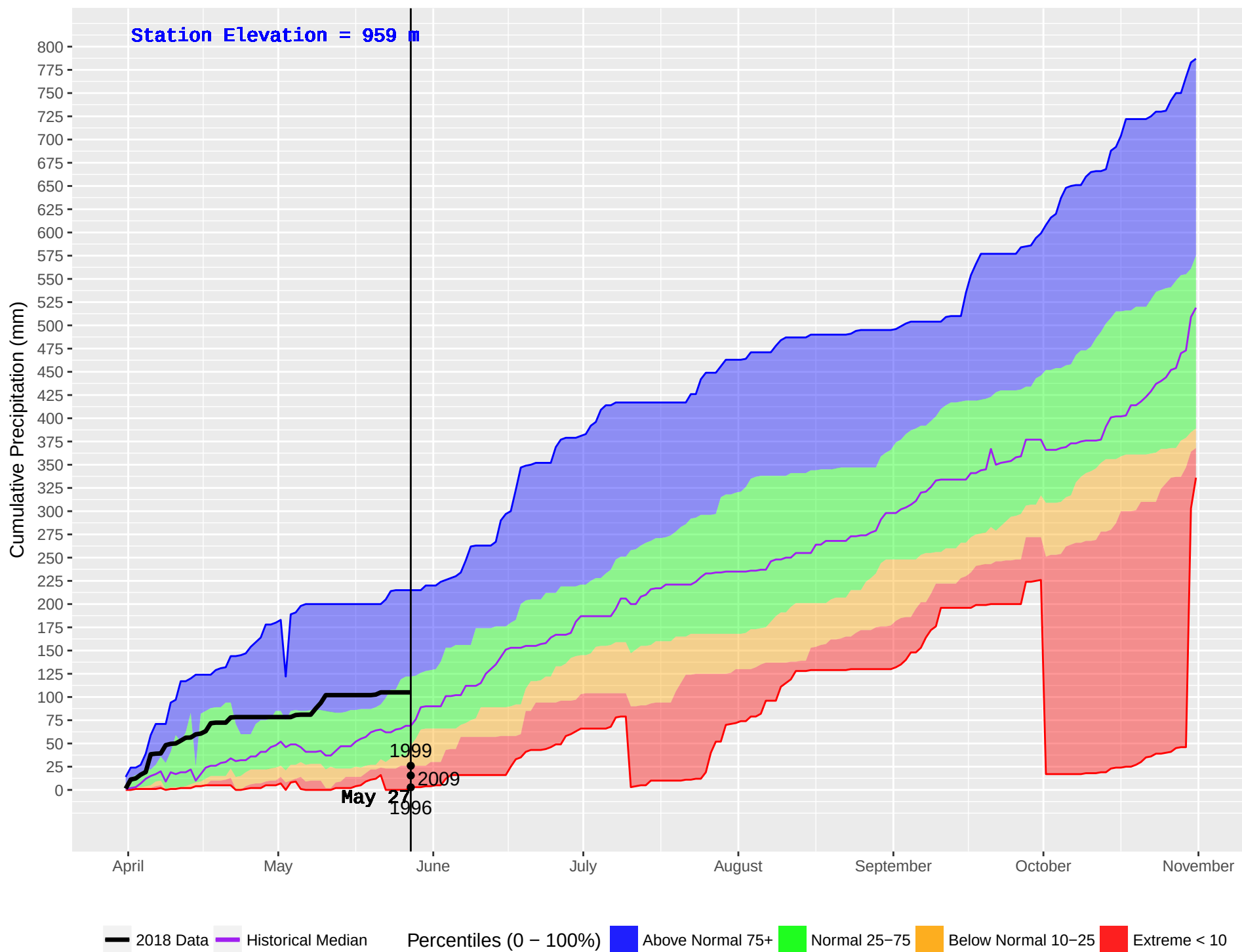
WELLS GRAY (266) : Historical (1994–2016) and Current (2018) Noon Cumulative Precipitation
