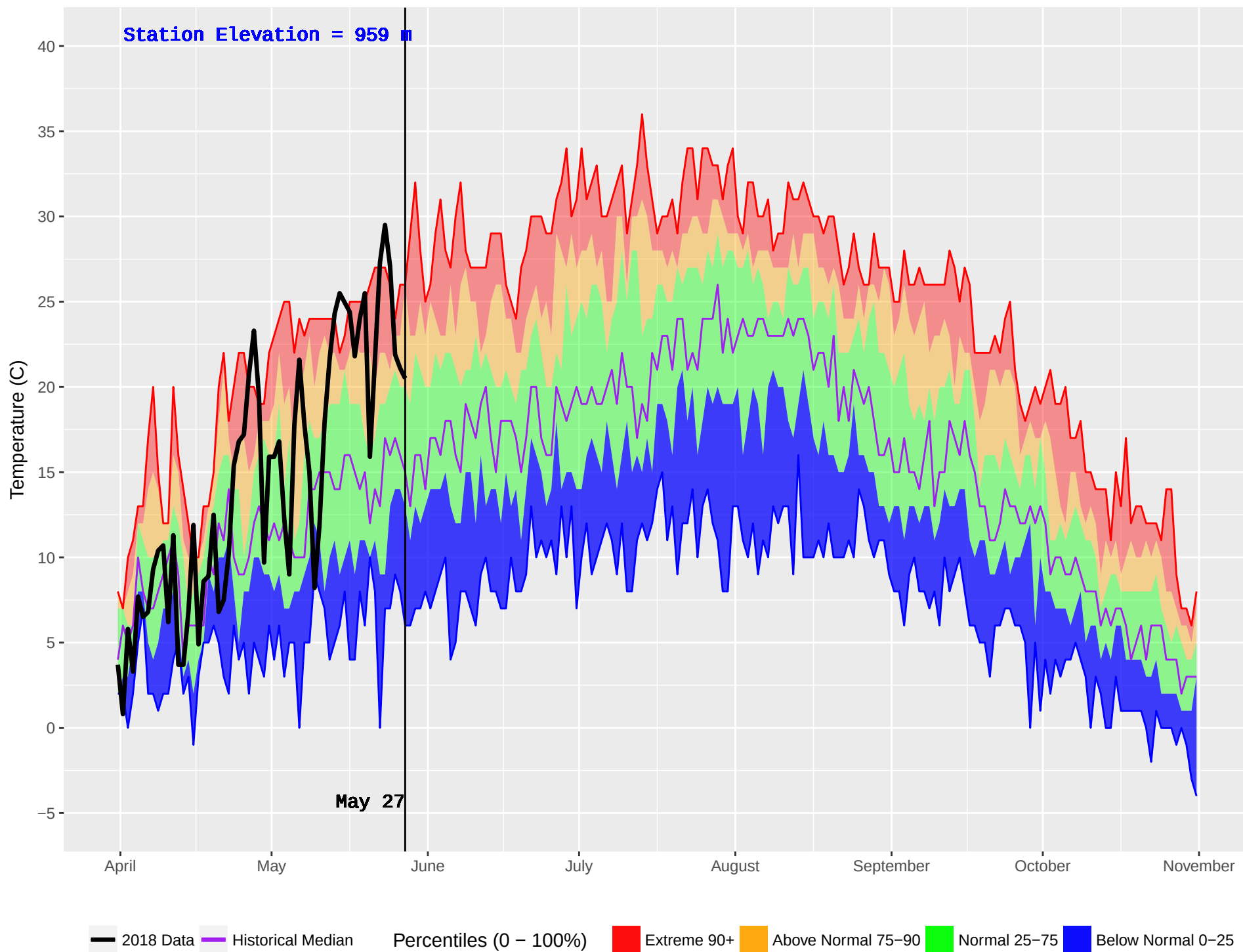
WELLS GRAY (266) : Historical (1994–2016) and Current (2018) Noon Temperature
