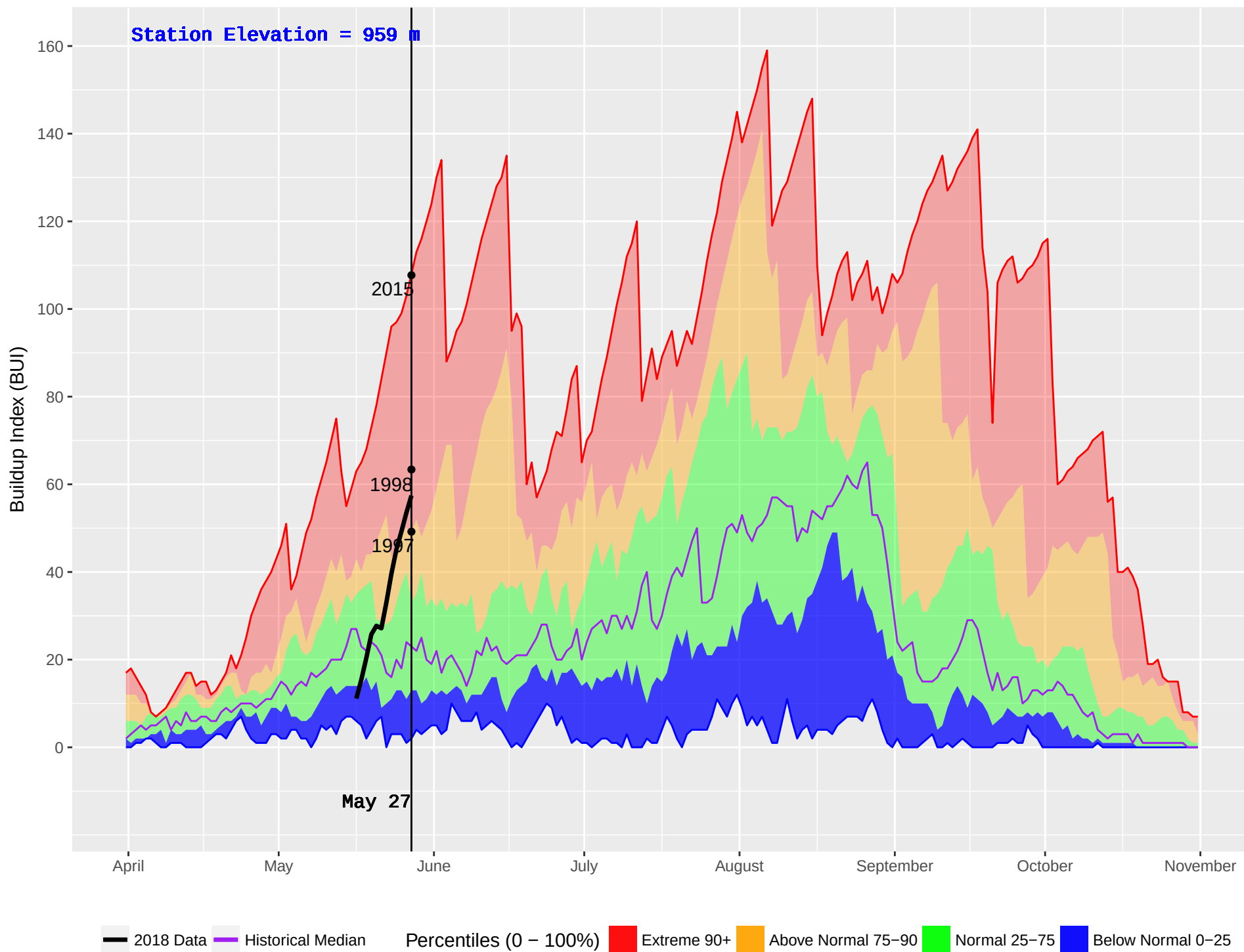
WELLS GRAY (266) : Historical (1994–2016) and Current (2018) Noon Buildup Index (BUI)
