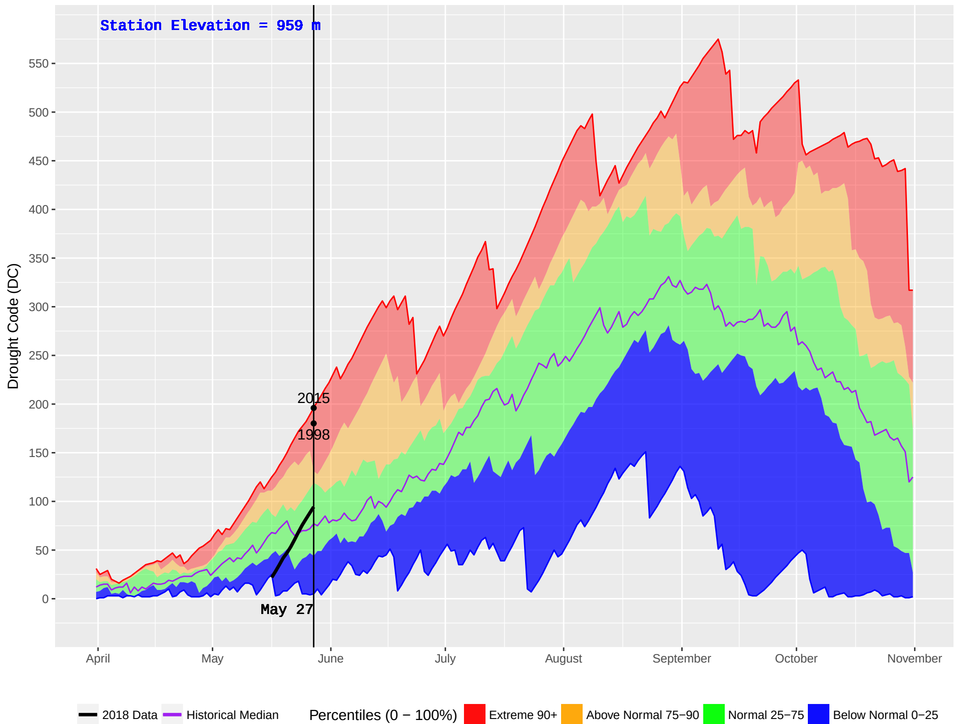
WELLS GRAY (266) : Historical (1994–2016) and Current (2018) Noon Drought Code (DC)
